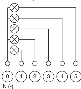
As signal tower
